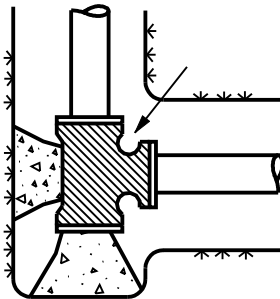
PLUGGED TEE
