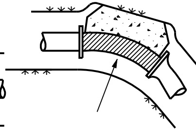
VERTICAL BEND
