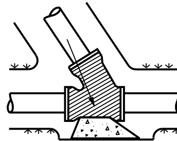
PLUGGED WYE
