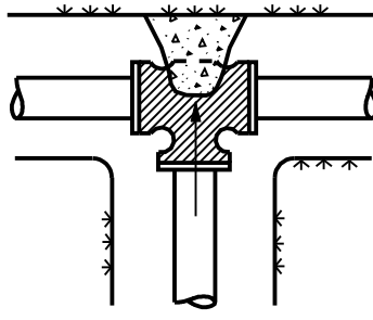
PLUGGED TEE
