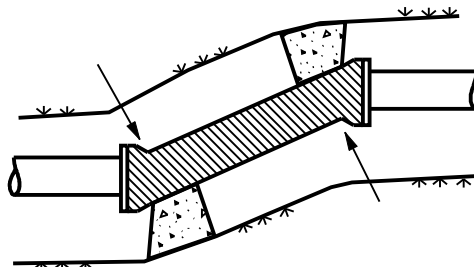
VERTICAL BEND
