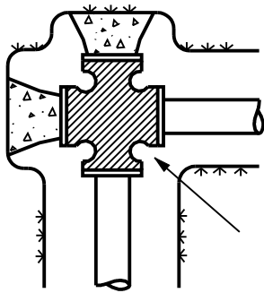
PLUGGED CROSS
