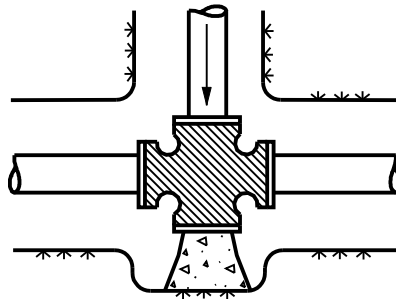
PLUGGED CROSS
